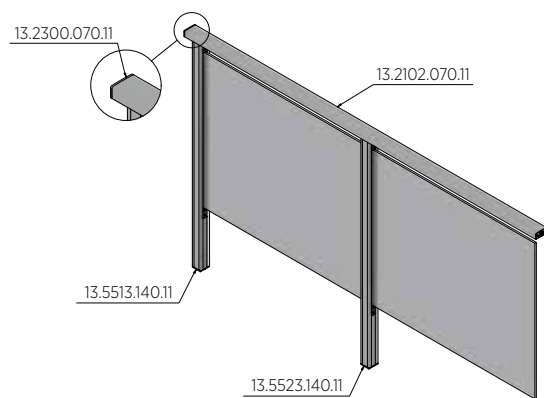
Side Handrail
